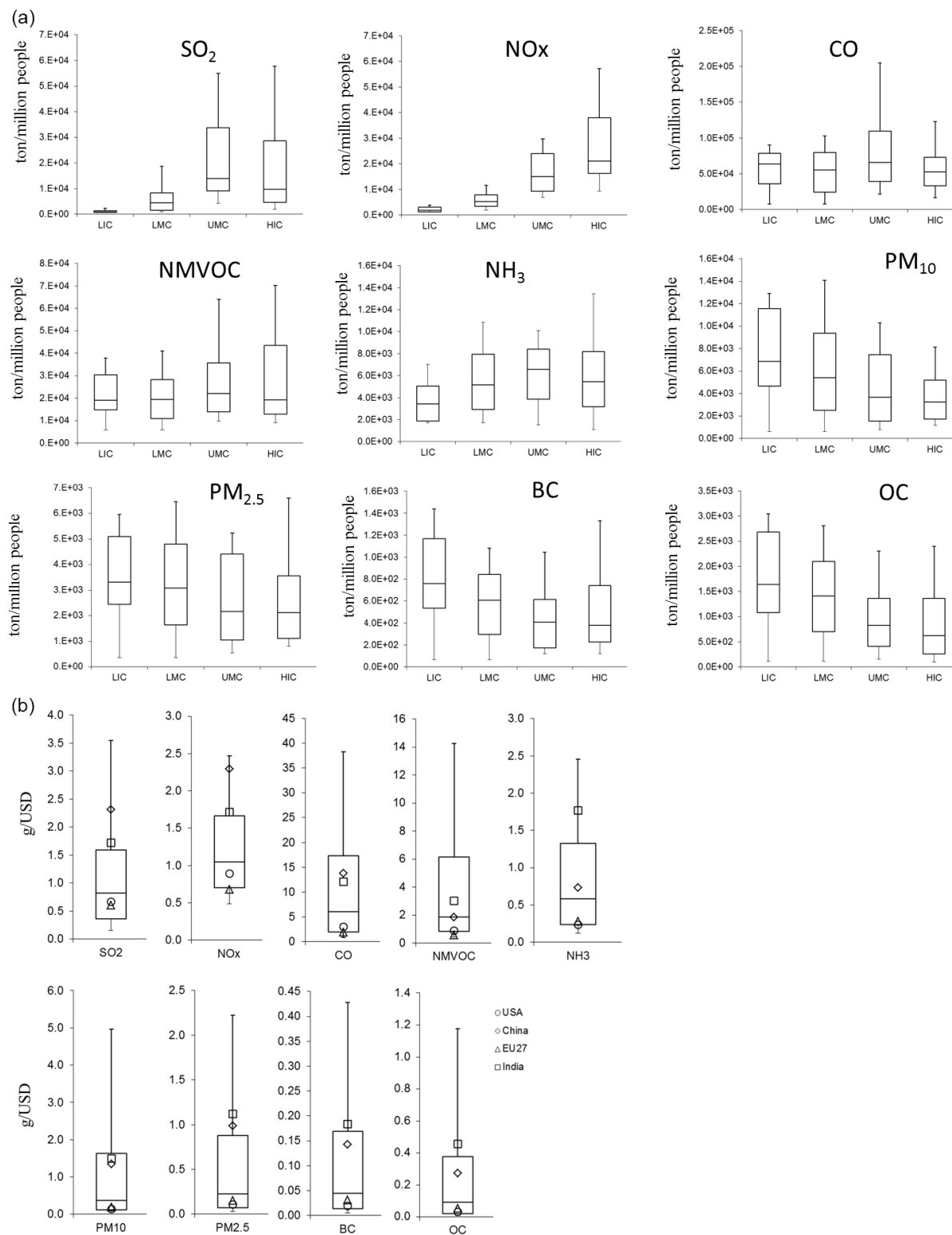
Figure 3. (a) 2010 per capita emissions per substance and per group of countries: low income (LIC), lower middle income (LMC), upper middle income (UMC) and high income (HIC) with the maximum, and minimum and the percentiles reported in the box plot (10, 50 and 90°) and the maximum and minimum in each group of countries. (b) Pollutant specific emissions divided by GDP ( \text{g USD}^{-1} ) for the year 2010. Percentiles are reported in the box plots (10, 25, 50, 75 and 90°) together with emission/GDP for specific regions (EU27, USA, China and India).
