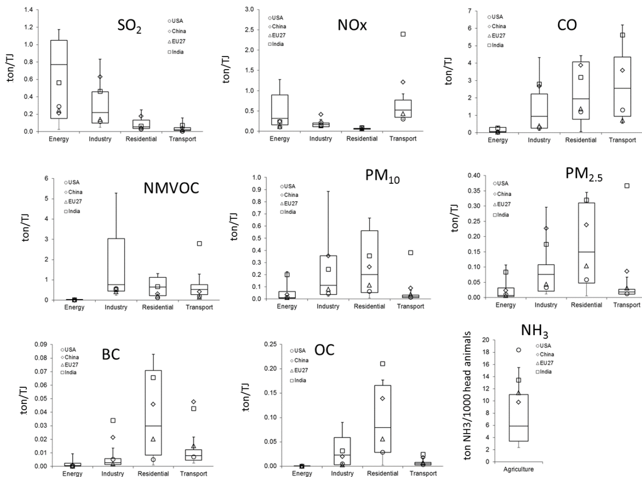
Figure 4. Sector specific implied emissions factors ( \text{ton/TJ}^{-1} ) for the year 2010. Percentiles are reported in the box plots (10, 25, 50, 75, and 90 o ) together with implied emission factors for specific regions (EU27, USA, China and India). Note – For the percentiles the following countries are left out. For CO – for the industry sector: Togo, Eritrea, Congo, Côte d’Ivoire, Kenya, Benin; for the residential sector: Maldives; for the transport sector: North Korea, Afghanistan, Laos, Tajikistan, Mongolia. For \text{SO}_2 – for the industry sector: Namibia, Laos, Jamaica. For \text{NO}_x – for the residential sector: Maldives; for the TRANSPORT sector: Afghanistan, Laos, North Korea, Tajikistan. For NMVOC – for the energy sector: Bhutan; for the industry sector: Togo, Eritrea, Côte d’Ivoire, Congo, Cameroon, Kenya, Benin, Aruba, Antigua, Bahamas, Ethiopia, Sudan, Senegal, Equatorial Guinea, Central African Rep., Sri Lanka, Angola, Mozambique, Zambia, Jamaica; for the residential sector: American Samoa, Gum, Maldives, Tonga; for the transport sector: Afghanistan, Laos, North Korea. For \text{PM}_{10} – for the industry sector: Togo, Eritrea, Côte d’Ivoire, Congo, Kenya, Benin, for the transport sector: Afghanistan. For \text{PM}_{2.5} – for the energy sector: Tajikistan, Luxembourg; for the industry sector: Togo and Eritrea; for the transport sector: Afghanistan. For BC – for the energy sector: Nigeria, Malaysia, Belgium, Oman, Finland, Georgia, Vietnam, Canada, Armenia, Tunisia, Jordan, The Netherlands, Trinidad and Tobago, Algeria, Latvia, United Arab Emirates, Brunei, Turkmenistan, Japan, Mozambique, Congo, Qatar, Bahrain, Moldova, Kyrgyzstan, South Korea, Taiwan, Luxembourg, Bhutan, Tajikistan; for the industry sector: Trinidad and Tobago, Malta; for the transport sector: Afghanistan. For OC – for the energy sector: Tunisia, Jordan, Trinidad and Tobago, Algeria, United Arab Emirates, Brunei, Turkmenistan, Tajikistan, Mozambique, Congo, Qatar, Bahrain, Kyrgyzstan, Taiwan, Myanmar, South Korea, Vietnam; for the industry sector: Bahrain, Eritrea; for the residential sector: Greenland, Gibraltar, Faroe Islands, Saint Pierre et Miquelon; for the transport sector: Afghanistan. For \text{NH}_3 – for the agriculture sector: Faroe Islands, Tajikistan, Greenland, Falkland Islands, Kyrgyzstan, South Korea, Brunei, American Samoa, Malaysia, Trinidad and Tobago, Bahamas, Saint Pierre et Miquelon, Sri Lanka, Suriname, Réunion, Thailand, Indonesia, Japan, Barbados, Bhutan, Guyana, Costa Rica.
