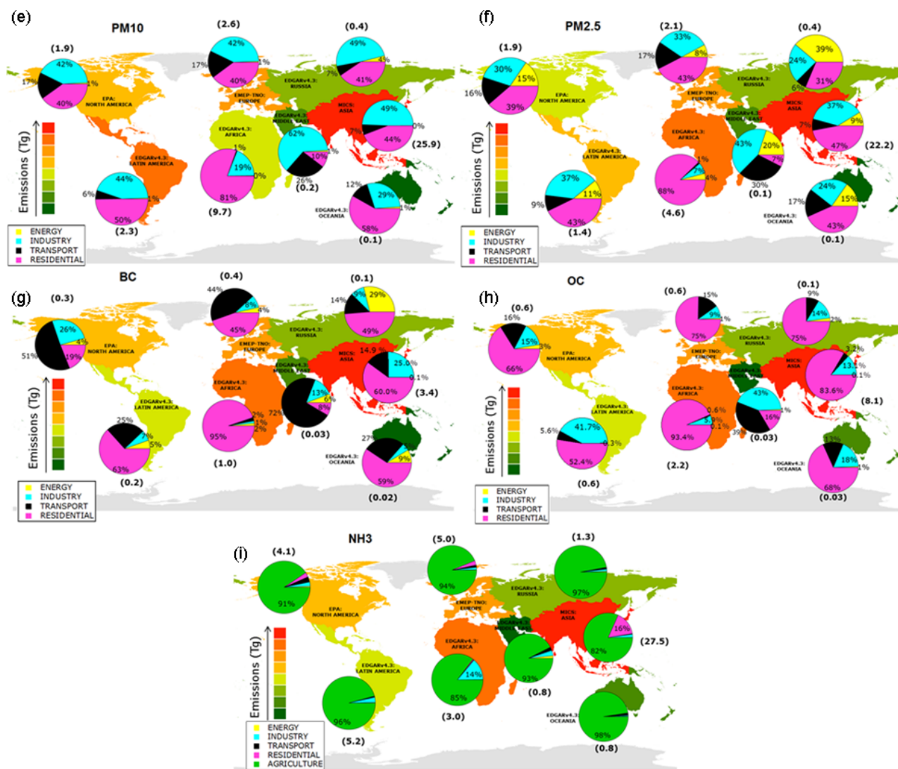
Figure 2. Sector-specific breakdown of regional emission totals (Tg) for 2010: (a) SO 2 , (b) NO x , (c) CO, (d) NMVOC, (e) PM 10 , (f) PM 2.5 , (g) BC, (h) OC and (i) NH 3 .
