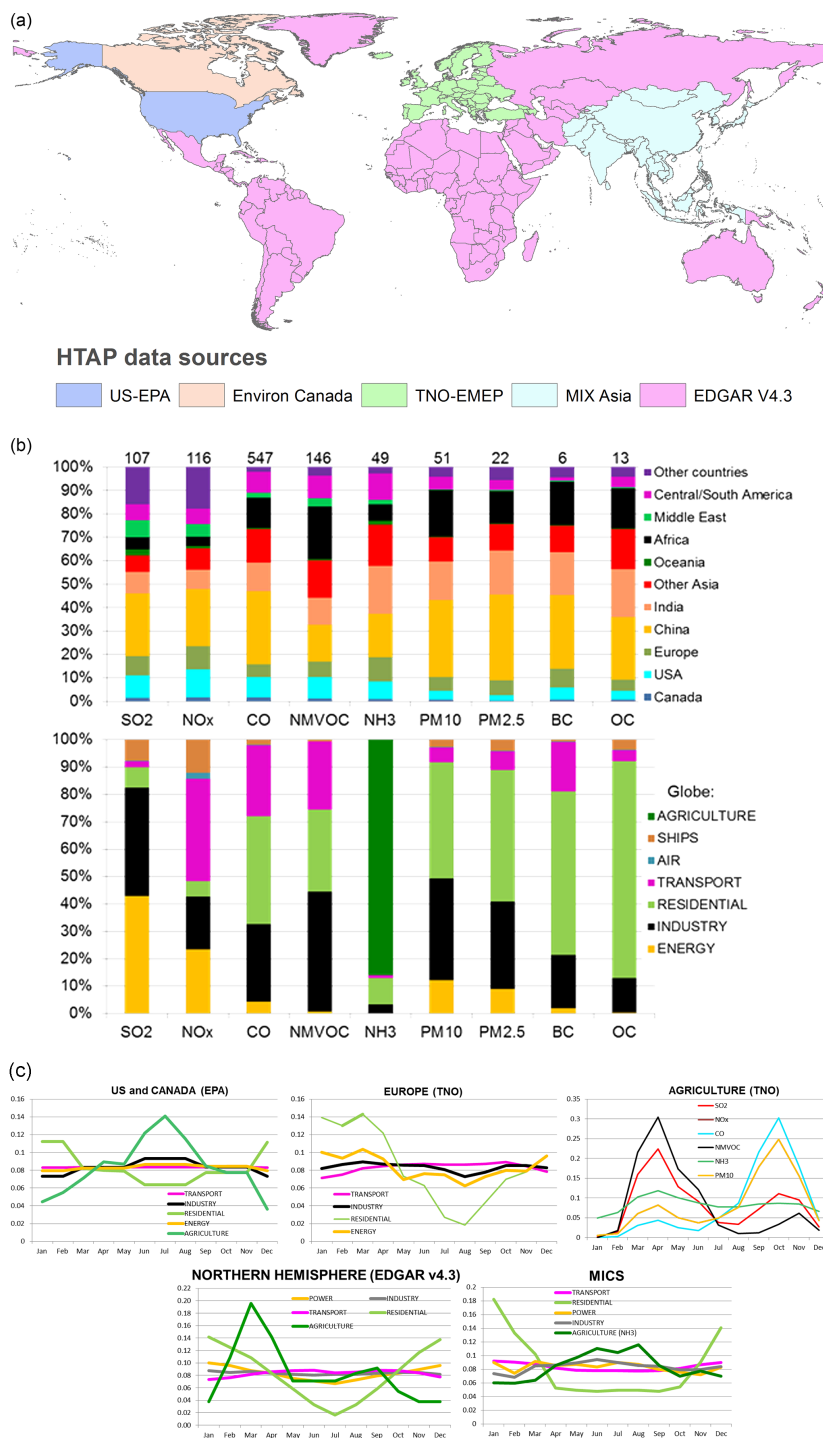
Figure 1. (a) Collection of regional emission inventories (US-EPA, Environ Canada, TNO-EMEP, MIX (MICS-Asia III), EDGARv4.3 for the global air pollutants and their use for world countries in data set HTAP v2.2 (b) Regional relative contribution to 2010 pollutant emissions (upper panel). Asian emissions have been divided into China, India and other Asia fractions from the MIX database. The region “rest of the world” has been disaggregated into Oceania, Africa, Middle East, Central/South America and other countries making use of the EDGAR v4.3 inventory. Global sector-specific anthropogenic emissions of gaseous pollutants and particulate matter components for the year 2010 (lower panel). Global absolute emissions are reported on top of each bar in Tg species per year. Large scale open-biomass burning is not included in the analysis. (c) Temporal profiles with relative factors varying around 1/12 and applied on the yearly emissions of the different data sources (US-EPA for US and Canada, EMEP-TNO for Europe with compound-specific variation of the agricultural temporal profiles, EDGAR temporal profiles for the Northern Hemisphere and MICS profiles for Asia).
